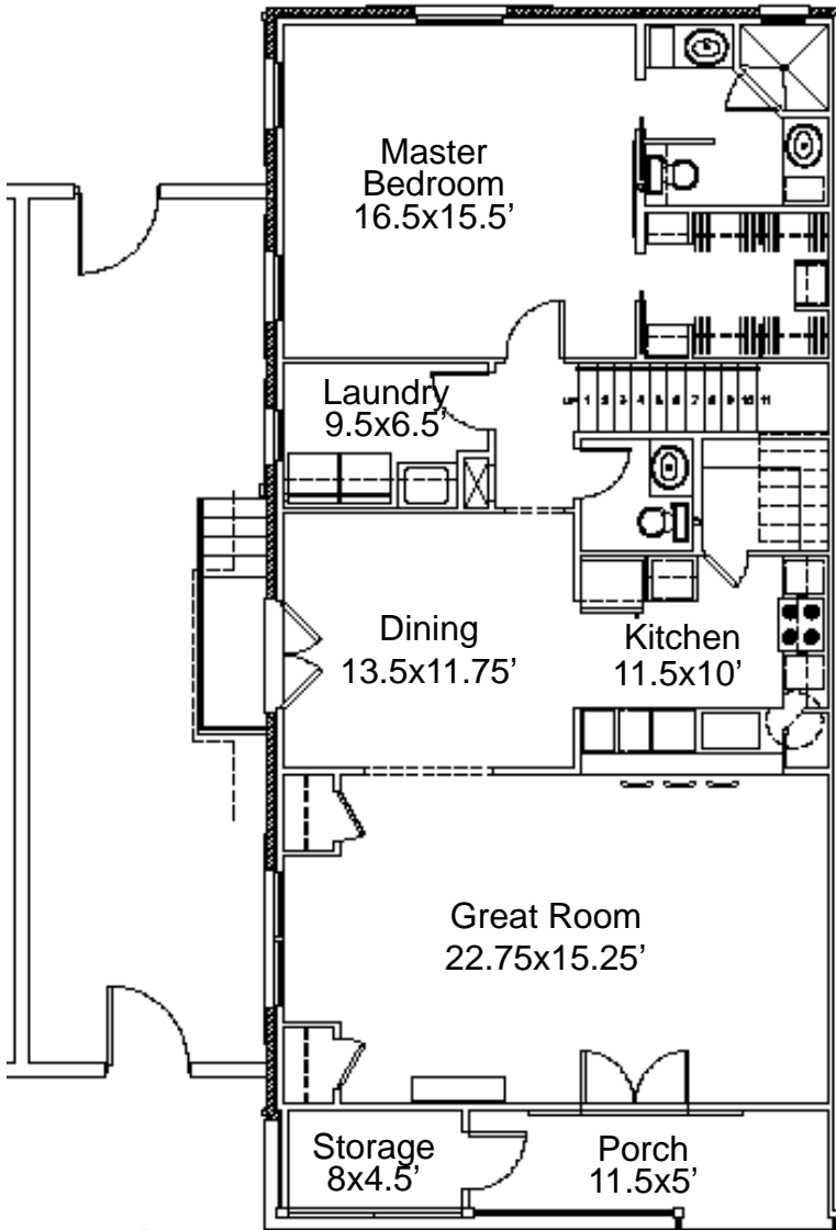
First Floor
